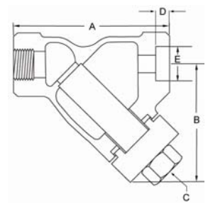
Bolted Cover
