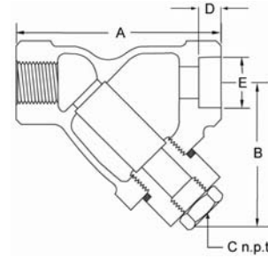
Threaded Cover
