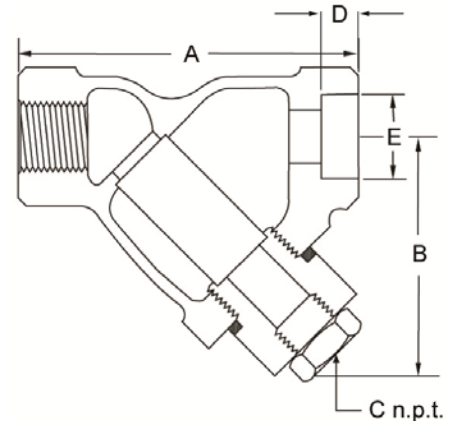
Model 600YTSS (Threaded) – Stainless Steel Model 600YSWS (Socket Weld) – Stainless Steel
